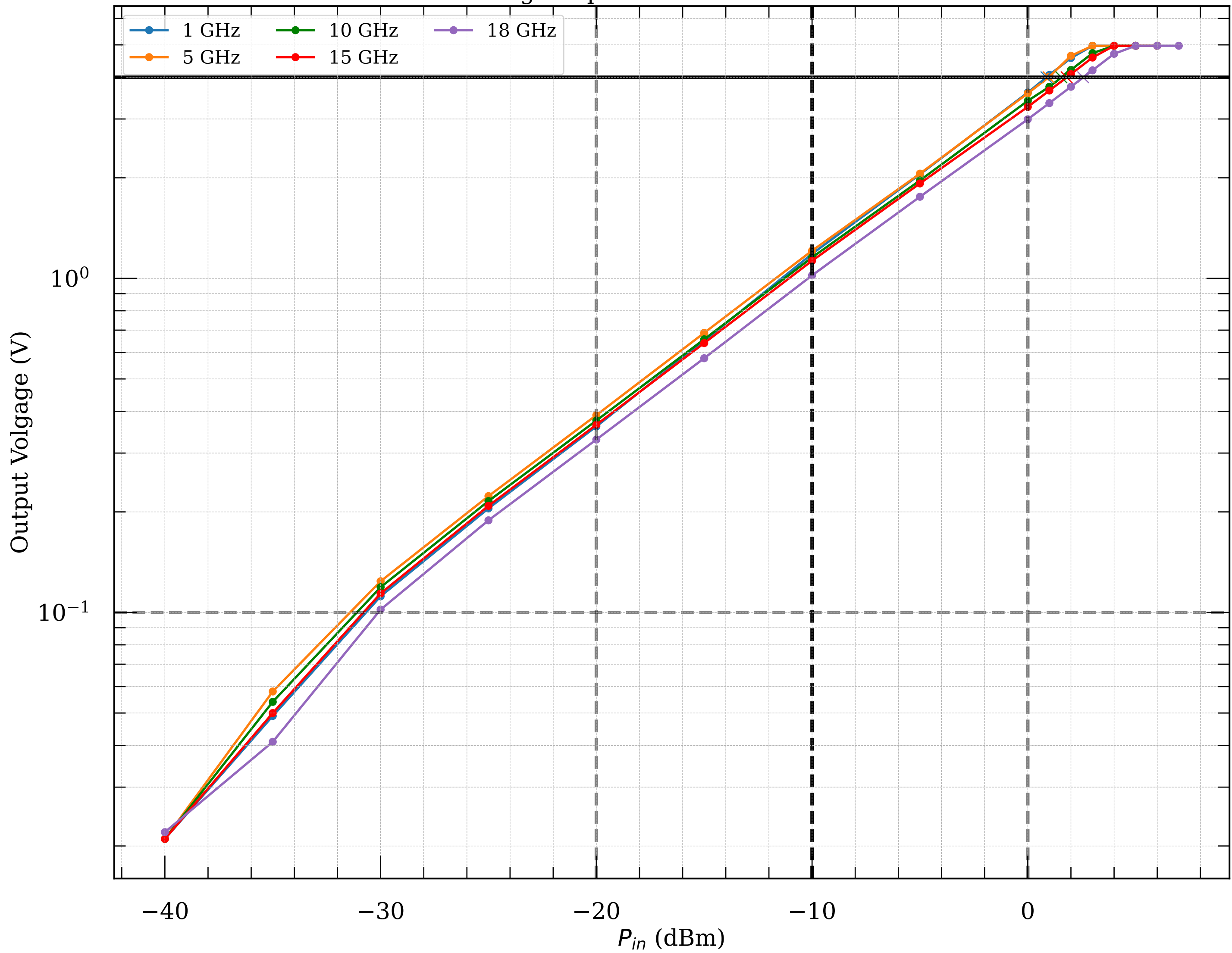
Measured voltage-to-power curve of detector module088
